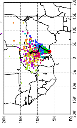
Ballons laches a J+18 h (05/05, 6 UTC)
