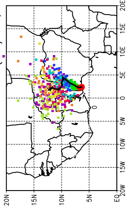
Ballons laches a J+12 h (05/05, 00 UTC)
