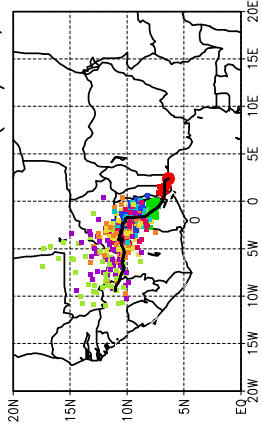
Ballons laches a J+12 h (11/05, 12 UTC)
