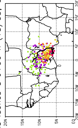
Ballons laches a J+96 h (15/05, 00 UTC)
