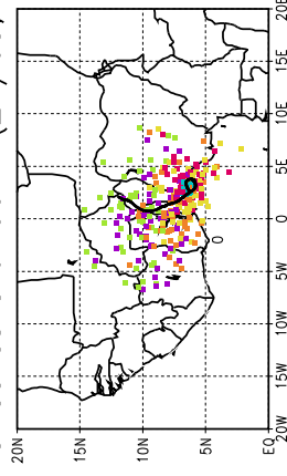
Ballons laches a J+90 h (21/05, 6 UTC)
