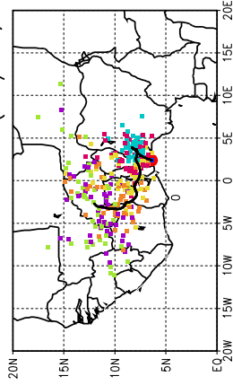
Ballons laches a J+72 h (20/05, 12 UTC)
