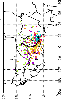
Ballons laches a J+78 h (20/05, 18 UTC)
