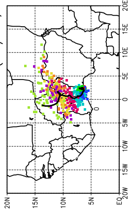
Ballons laches a J+24 h (22/05, 00 UTC)
