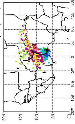
Ballons laches a J+18 h (21/05, 18 UTC)
