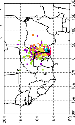
Ballons laches a J+72 h (26/05, 00 UTC)
