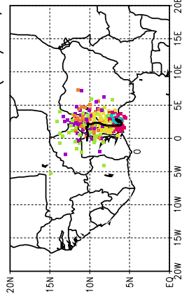
Ballons laches a J+78 h (26/05, 6 UTC)
