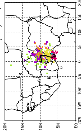
Ballons laches a J+90 h (26/05, 18 UTC)
