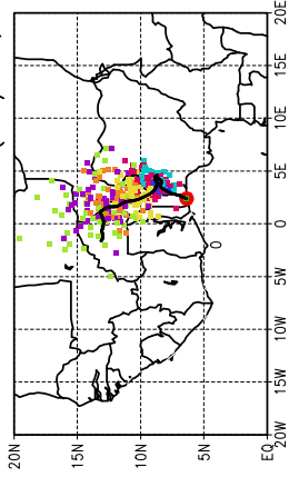
Ballons laches a J+48.h (25/05, 00 UTC)
