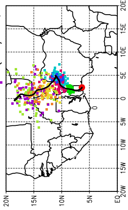
Ballons laches a J+24 h (24/05, 12 UTC)
