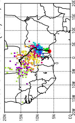
Ballons laches a J+36 h (05/06, 00 UTC)
