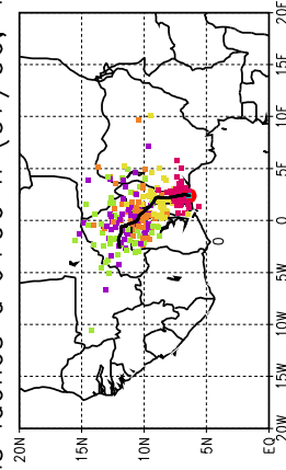
Ballons laches a J+96 h (07/06, 12 UTC)
