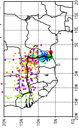
Ballons laches a J+18 h (06/06, 18 UTC)
