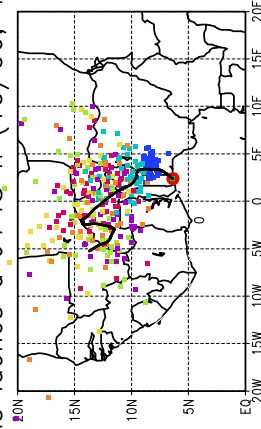
Ballons laches a J+48 h (10/06, 12 UTC)
