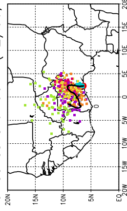
Ballons laches a J+90 h (12/06, 6 UTC)
