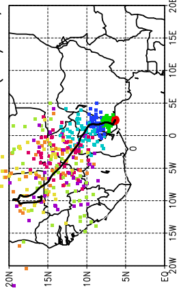
Ballons laches a J+18 h (09/06, 6 UTC)
