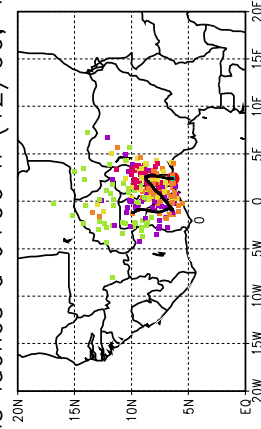
Ballons laches a J+96 h (12/06, 12 UTC)
