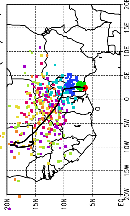
Ballons laches a J+30 h (09/06, 18 UTC)
