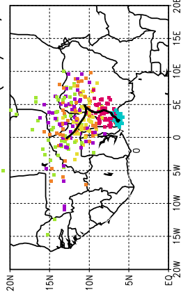
Ballons laches a J+78. h (14/06, 18 UTC)
