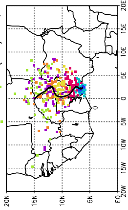
Ballons laches a J+60. h (14/06, 00 UTC)
