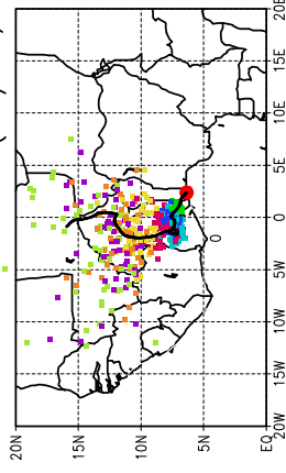
Ballons laches a J+30 h (12/06, 18 UTC)
