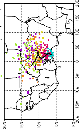
Ballons laches a J+72. h (14/06, 12 UTC)
