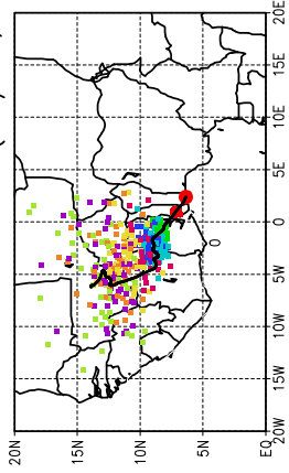
Ballons laches a J+12 h (12/06, 00 UTC)
