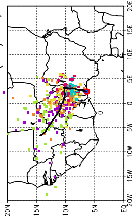
Ballons laches a J+72 h (19/06, 12 UTC)
