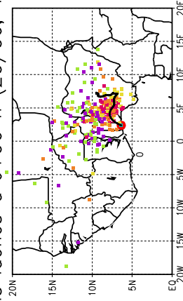
Ballons laches a J+96 h (20/06, 12 UTC)
