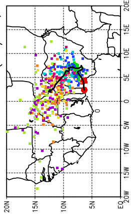
Ballons laches a J+12 h (17/06, 00 UTC)
