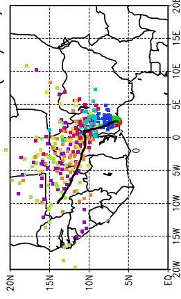
Ballons laches a J+42 h (18/06, 6 UTC)
