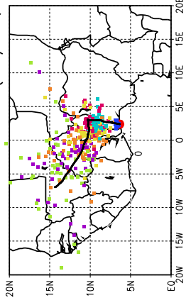
Ballons laches a J+66 h (19/06, 6 UTC)
