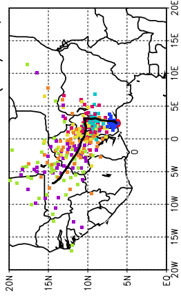
Ballons laches a J+60 h (19/06, 00 UTC)
