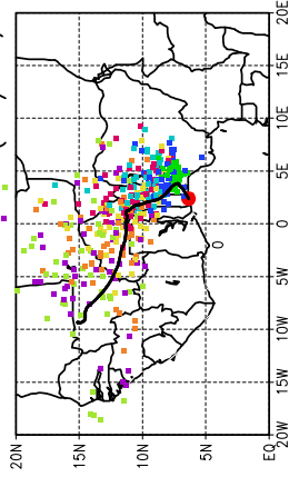
Ballons laches a J+24 h (17/06, 12 UTC)
