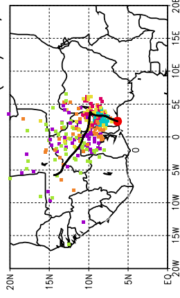
Ballons laches a J+78 h (19/06, 18 UTC)
