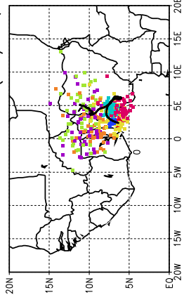
Ballons laches a J+66 h (20/06, 6 UTC)
