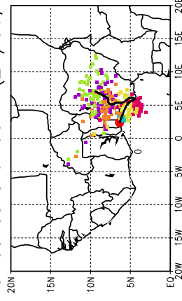
Ballons laches a J+90 h (21/06, 6 UTC)
