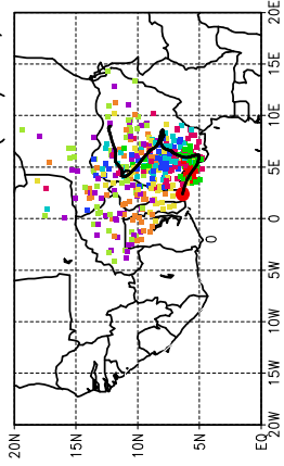
Ballons laches a J+12 h (18/06, 00 UTC)
