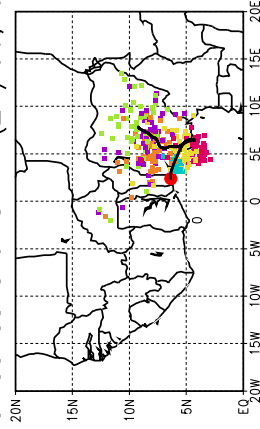
Ballons laches a J+84 h (21/06, 00 UTC)
