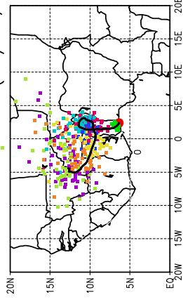
Ballons laches a J+42 h (19/06, 6 UTC)
