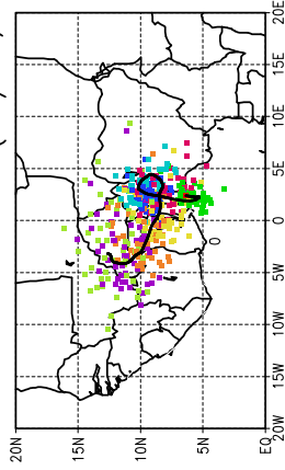
Ballons laches a J+24 h (18/06, 12 UTC)
