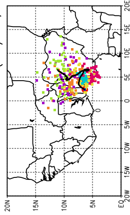
Ballons laches a J+72 h (20/06, 12 UTC)
