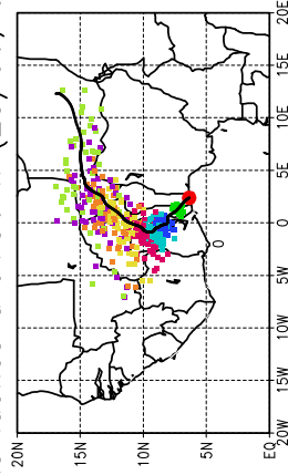
Ballons laches a J+36 h (23/06, 00 UTC)
