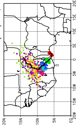
Ballons laches a J+12 h (22/06, 00 UTC)
