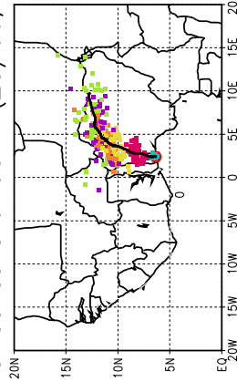
Ballons laches a J+90 h (25/06, 6 UTC)
