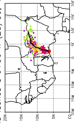
Ballons laches a J+96 h (25/06, 12 UTC)
