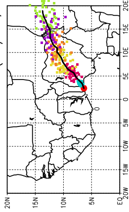
Ballons laches a J+84 h (02/07, 00 UTC)
