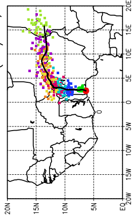
Ballons laches a J+36 h (30/06, 00 UTC)
