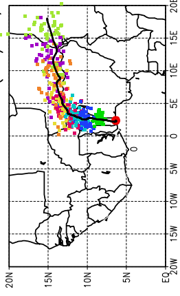
Ballons laches a J+18 h (29/06, 6 UTC)
