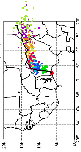
Ballons laches a J+24 h (30/06, 00 UTC)
