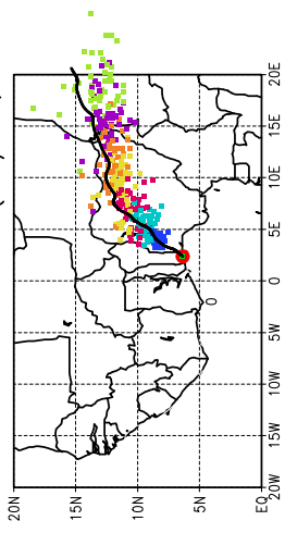
Ballons laches a J+48 h (01/07, 00 UTC)
