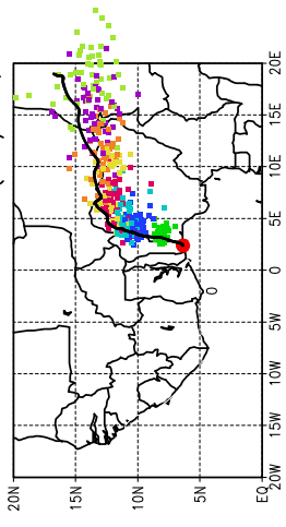
Ballons laches a J+30 h (30/06, 6 UTC)
