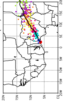
Ballons laches a J+66 h (01/07, 18 UTC)
