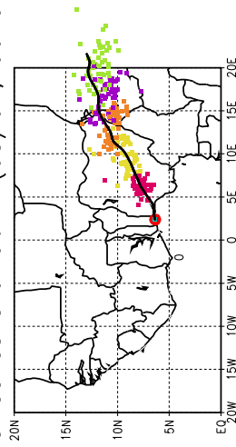
Ballons laches a J+96 h (03/07, 00 UTC)
