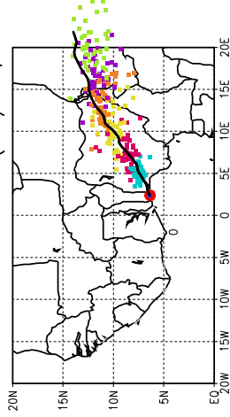
Ballons laches a J+72 h (02/07, 00 UTC)
