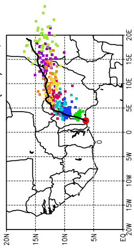
Ballons laches a J+36 h (30/06, 12 UTC)
