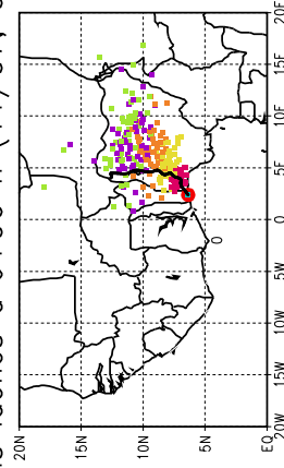
Ballons laches a J+96 h (11/07, 00 UTC)
