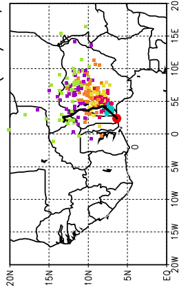
Ballons laches a J+78 h (10/07, 6 UTC)
