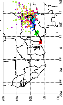
Ballons laches a J+18 h (07/07, 18 UTC)
