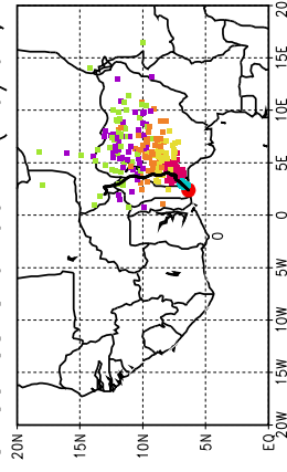
Ballons laches a J+90 h (10/07, 18 UTC)
