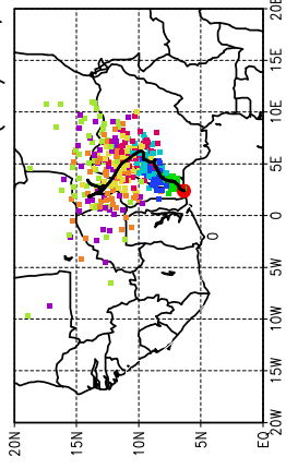
Ballons laches a J+18 h (10/07, 6 UTC)
