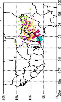
Ballons laches a J+72 h (12/07, 12 UTC)
