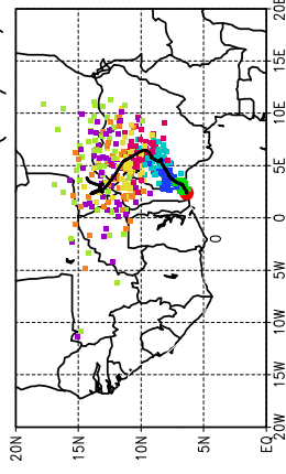
Ballons laches a J+30 h (10/07, 18 UTC)
