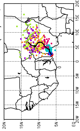
Ballons laches a J+60 h (12/07, 00 UTC)
