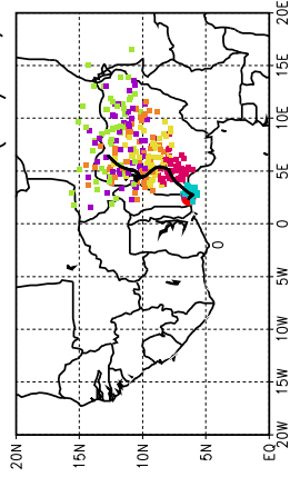
Ballons laches a J+84 h (13/07, 00 UTC)
