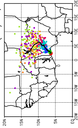
Ballons laches a J+36 h (11/07, 00 UTC)
