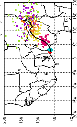
Ballons laches a J+90 h (16/07, 6 UTC)
