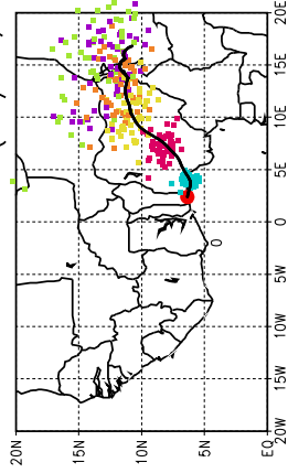
Ballons laches a J+84 h (16/07, 00 UTC)
