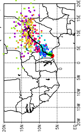
Ballons laches a J+36 h (14/07, 00 UTC)
