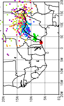
Ballons laches a J+18 h (16/07, 18 UTC)
