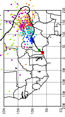
Ballons laches a J+42 h (18/07, 18 UTC)
