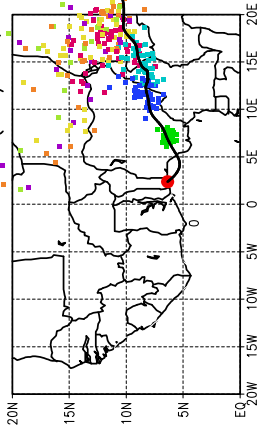
Ballons laches a J+24 h (22/07, 00 UTC)
