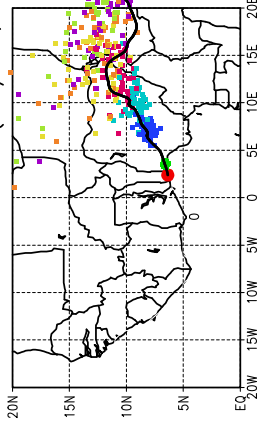
Ballons laches a J+42 h (22/07, 18 UTC)
