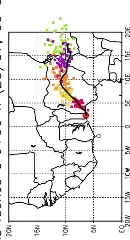
Ballons laches a J+96 h (25/07, 00 UTC)
