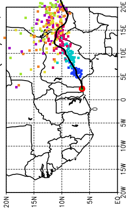
Ballons laches a J+48 h (23/07, 00 UTC)
