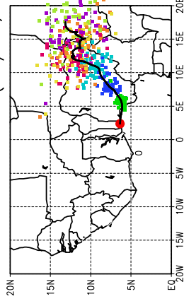
Ballons laches a J+30 h (22/07, 18 UTC)
