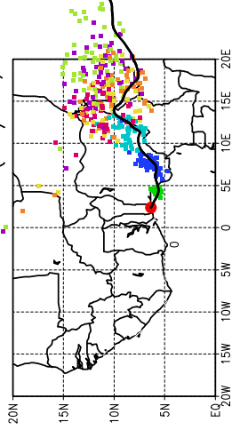
Ballons laches a J+36 h (23/07, 00 UTC)
