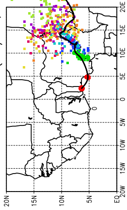
Ballons laches a J+12 h (22/07, 00 UTC)
