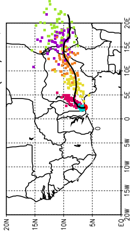
Ballons laches a J+84 h (26/07, 00 UTC)
