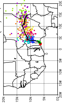
Ballons laches a J+36 h (25/07, 00 UTC)
