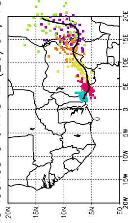
Ballons laches a J+78 h (26/07, 18 UTC)
