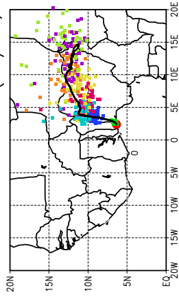
Ballons laches a J+42 h (25/07, 6 UTC)
