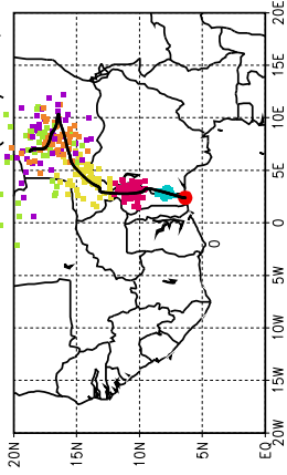
Ballons laches a J+84 h (07/05, 12 UTC)
