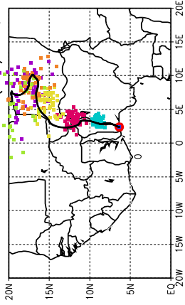
Ballons laches a J+72 h (07/05, 00 UTC)
