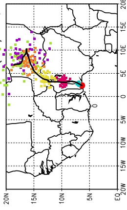
Ballons laches a J+90 h (07/05, 18 UTC)
