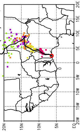
Ballons laches a J+96 h (09/05, 00 UTC)
