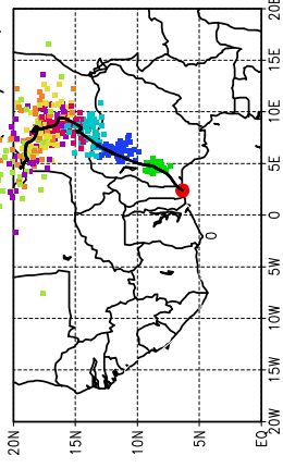
Ballons laches a J+30 (10/05, 18 UTC)
