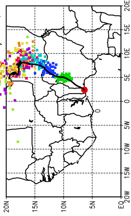
Ballons laches a J+24 (10/05, 12 UTC)
