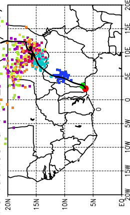
Ballons laches a J+42 h (14/05, 6 UTC)
