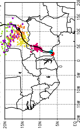
Ballons laches a J+90 h (16/05, 6 UTC)
