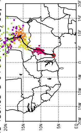
Ballons laches a J+96 h (16/05, 12 UTC)
