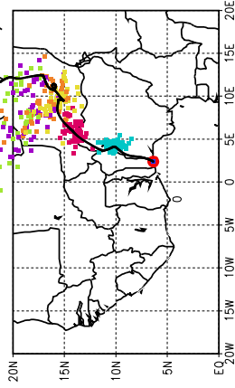
Ballons laches a J+72 h (15/05, 12 UTC)
