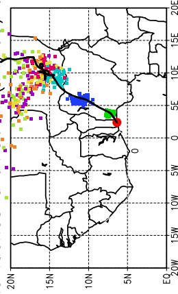
Ballons laches a J+36 h (14/05, 00 UTC)
