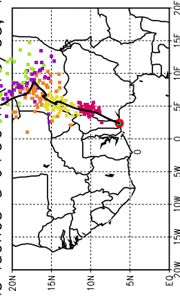
Ballons laches a J+96 h (18/05, 12 UTC)
