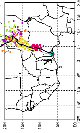
Ballons laches a J+90 h (18/05, 6 UTC)
