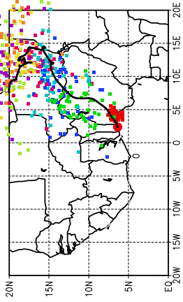
Ballons laches a J+12 h (20/05, 00 UTC)
