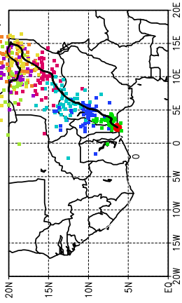
Ballons laches a J+36 h (21/05, 00 UTC)
