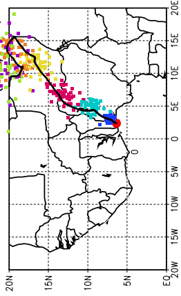
Ballons laches a J+60 h (22/05, 00 UTC)
