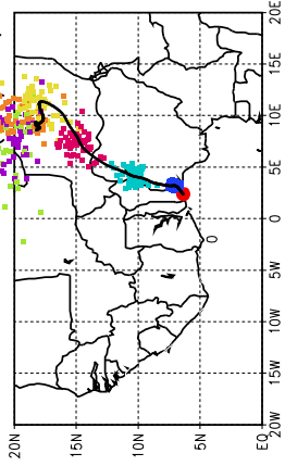
Ballons laches a J+60 h (23/05, 00 UTC)
