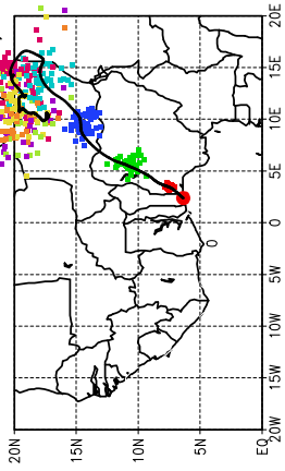
Ballons laches a J+12 h (23/05, 00 UTC)
