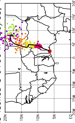
Ballons laches a J+96 h (26/05, 12 UTC)
