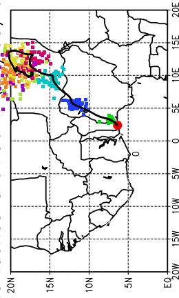
Ballons laches a J+36 h (24/05, 00 UTC)
