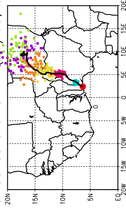
Ballons laches a J+84 h (26/05, 00 UTC)
