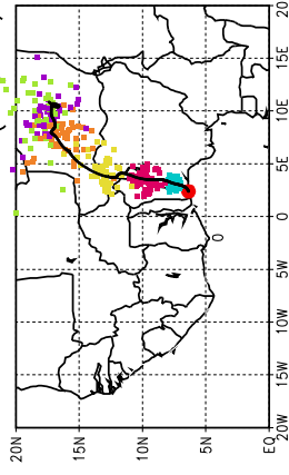
Ballons laches a J+78 h (30/05, 6 UTC)
