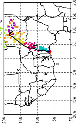
Ballons laches a J+66 h (30/05, 6 UTC)
