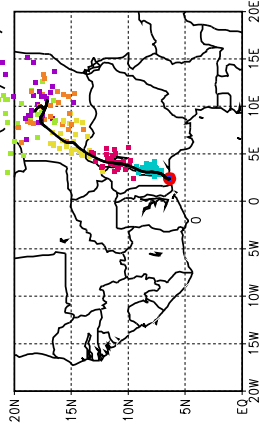
Ballons laches a J+72 h (30/05, 12 UTC)
