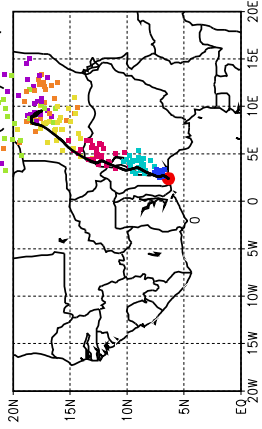
Ballons laches a J+60 h (30/05, 00 UTC)
