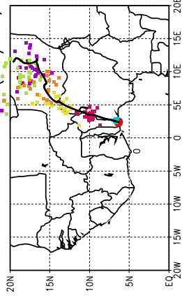
Ballons laches a J+90 h (31/05, 6 UTC)
