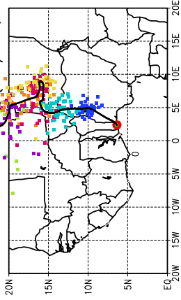
Ballons laches a J+48 (10/06, 12 UTC)
