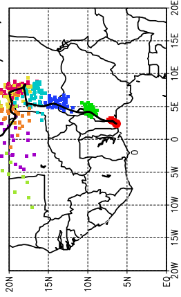
Ballons laches a J+10 (09/06, 00 UTC)
