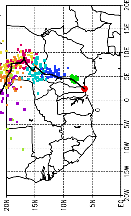
Ballons laches a J+30 (09/06, 18 UTC)
