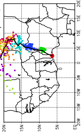
Ballons laches a J+21 (09/06, 12 UTC)
