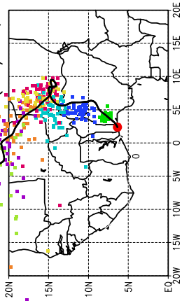
Ballons laches a 26 h (10/06, 12 UTC)
