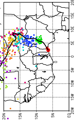
Ballons laches a 18 h (09/06, 18 UTC)
