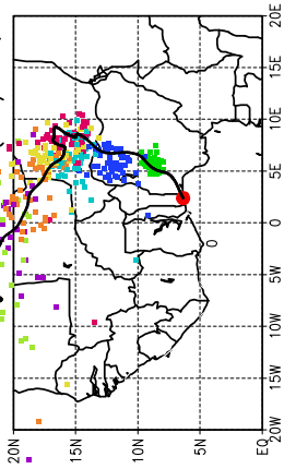
Ballons laches a 20 h (10/06, 00 UTC)
