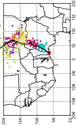
Ballons laches a J+72 h (13/06, 12 UTC)
