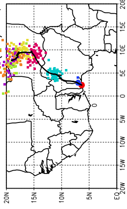
Ballons laches a J+66 h (15/06, 6 UTC)
