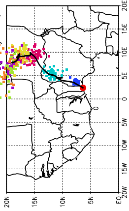
Ballons laches a J+60 h (15/06, 00 UTC)
