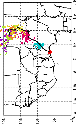
Ballons laches a J+78 h (15/06, 18 UTC)
