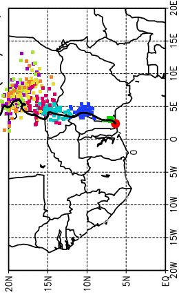
Ballons laches a J+42 h (18/06, 6 UTC)
