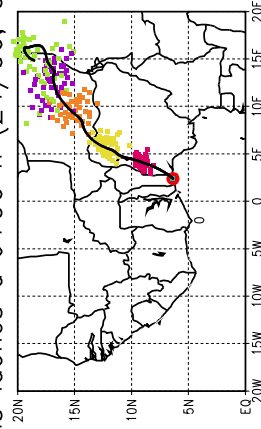
Ballons laches a J+96 h (24/06, 00 UTC)
