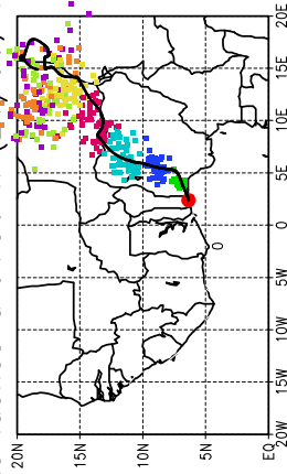
Ballons laches a J+36 h (21/06, 12 UTC)
