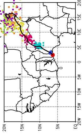
Ballons laches a J+66 h (01/07, 6 UTC)
