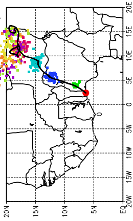
Ballons laches a J+36 h (30/06, 00 UTC)
