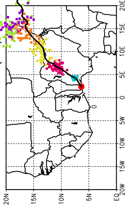
Ballons laches a J+84 h (02/07, 00 UTC)
