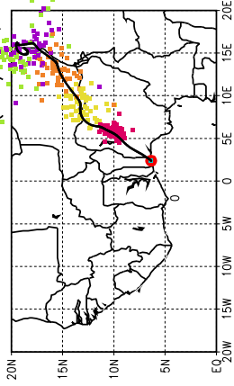
Ballons laches a J+96 h (02/07, 12 UTC)
