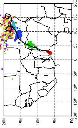
Ballons laches a J+18 h (29/06, 6 UTC)
