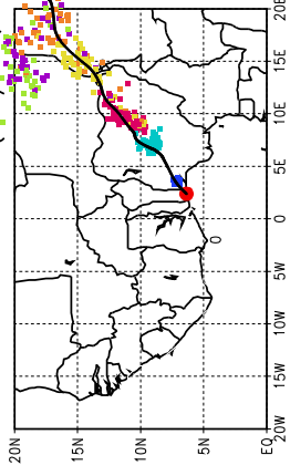
Ballons laches a J+66 h (02/07, 18 UTC)
