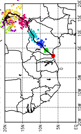
Ballons laches a J+36 h (01/07, 12 UTC)
