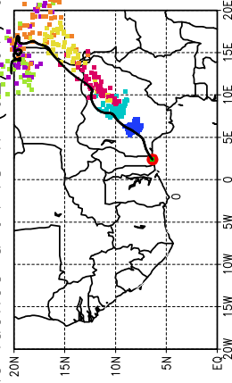
Ballons laches a J+48 h (02/07, 00 UTC)
