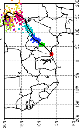
Ballons laches a J+24 h (01/07, 00 UTC)
