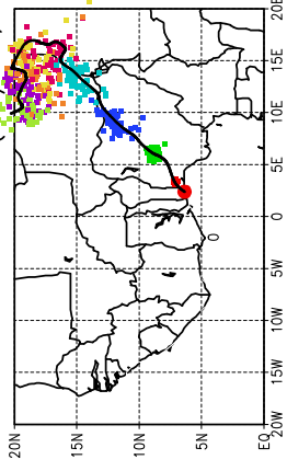
Ballons laches a J+18 h (01/07, 18 UTC)
