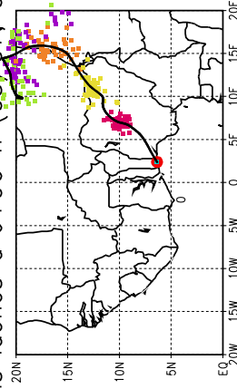
Ballons laches a J+96 h (05/07, 00 UTC)
