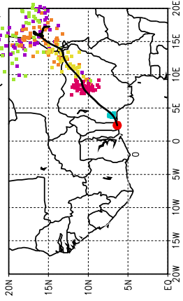
Ballons laches a J+90 h (06/07, 6 UTC)
