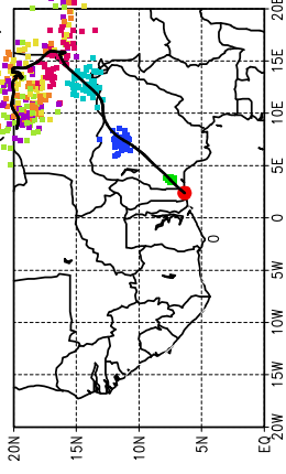
Ballons laches a J+42 h (04/07, 18 UTC)
