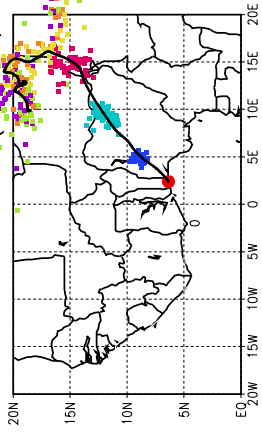
Ballons laches a J+60 h (05/07, 12 UTC)
