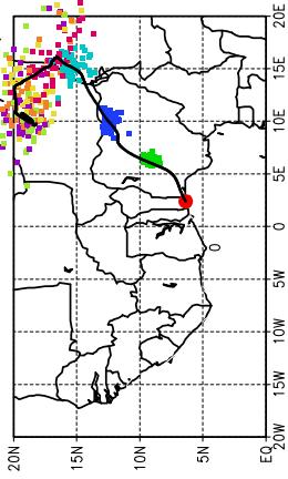
Ballons laches a J+24 h (04/07, 00 UTC)
