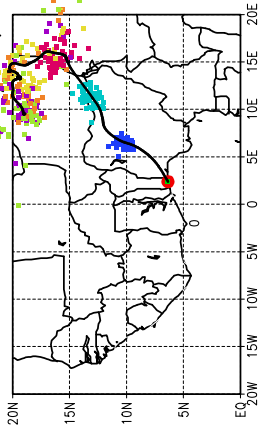
Ballons laches a J+48 h (05/07, 00 UTC)
