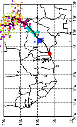
Ballons laches a J+48 h (06/07, 00 UTC)
