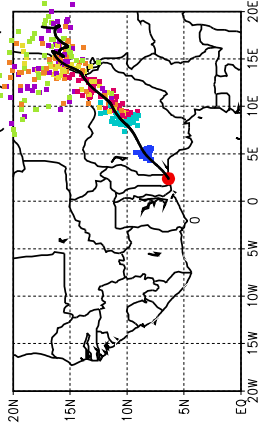
Ballons laches a J+60 h (06/07, 12 UTC)
