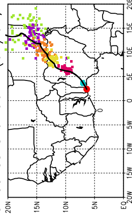
Ballons laches a J+90 h (07/07, 18 UTC)
