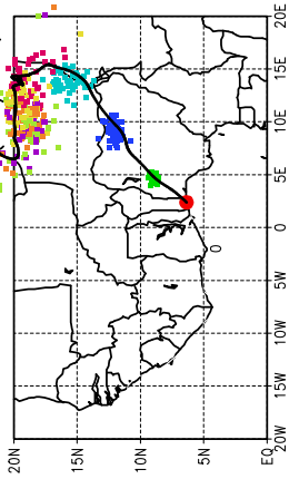
Ballons laches a J+36 h (05/07, 12 UTC)
