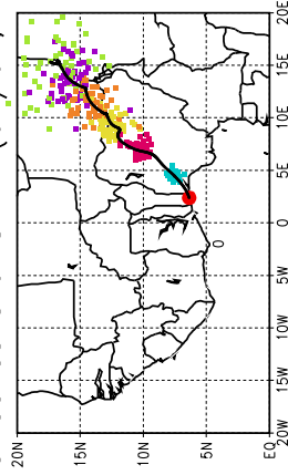
Ballons laches a J+84 h (07/07, 12 UTC)
