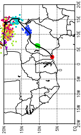
Ballons laches a J+24 h (05/07, 00 UTC)
