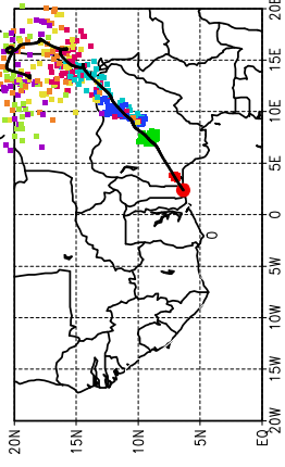
Ballons laches a J+18 h (06/07, 18 UTC)
