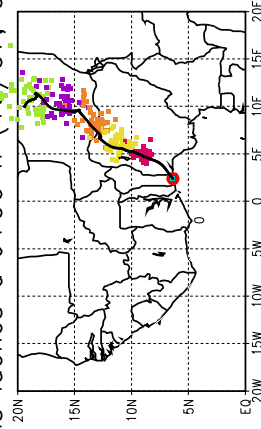
Ballons laches a J+96 h (10/07, 00 UTC)
