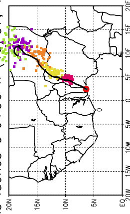
Ballons laches a J+96 h (10/07, 12 UTC)
