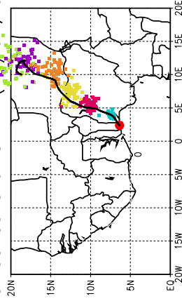
Ballons laches a J+84 h (10/07, 00 UTC)
