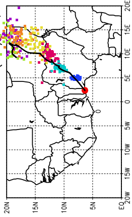
Ballons laches a J+60 h (09/07, 00 UTC)
