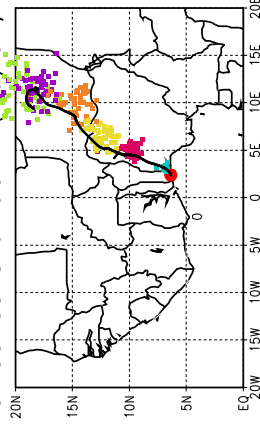
Ballons laches a J+90 h (10/07, 6 UTC)
