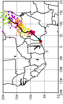
Ballons laches a J+90 h (12/07, 6 UTC)
