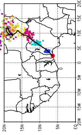
Ballons laches a J+60 h (11/07, 00 UTC)
