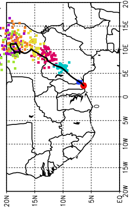
Ballons laches a J+66 h (11/07, 6 UTC)
