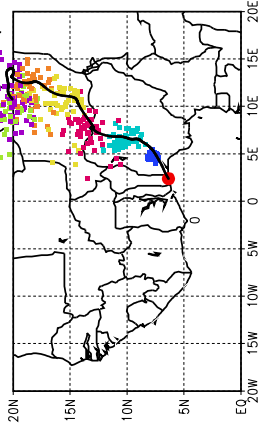
Ballons laches a J+60 h (13/07, 00 UTC)
