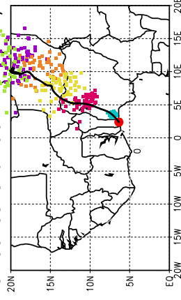
Ballons laches a J+90 h (14/07, 6 UTC)
