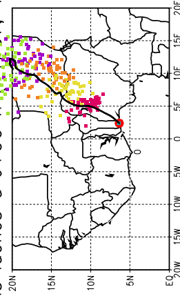
Ballons laches a J+96 h (14/07, 12 UTC)
